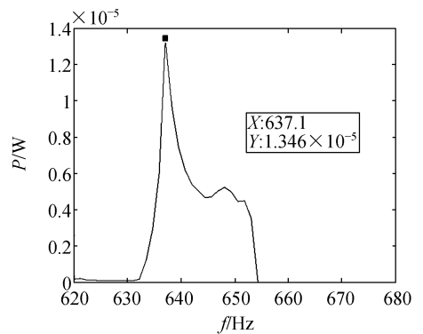
Fig. 6 Power output vs stimulation frequency
