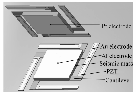
Fig. 1 Opened structure
